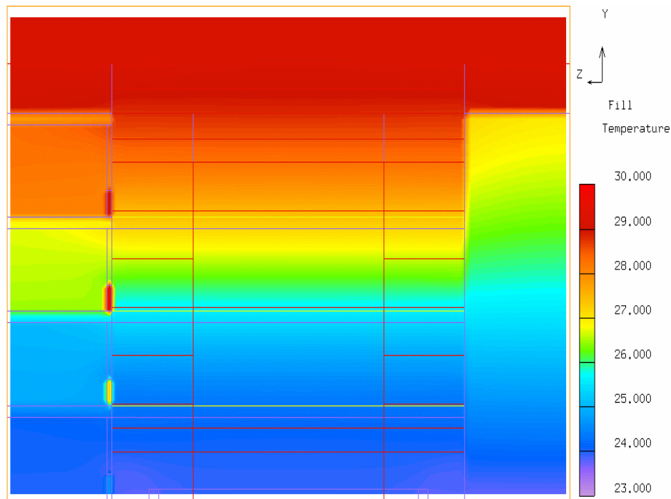
Figure 6 Diagram of temperatures, closed facades, North-South direction
